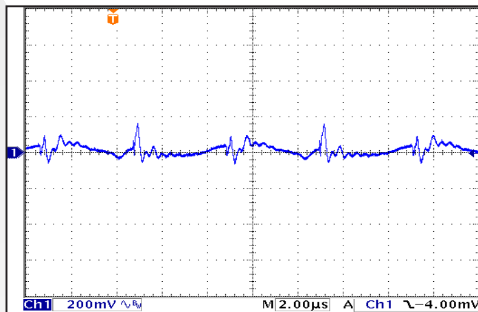
Figure 10: Output Voltage Ripple , Vout, at nominal input voltage and rated load current (200 mV/div). Load capacitance: 1 µF ceramic capacitor and 100 µF electrolytic capacitors. Bandwidth: 20 MHz. See Figure 13. Timescale: 2.00µsec/div.
