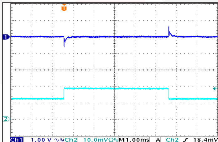
Figure 11: Output Voltage Response to Step-Change in Load Current , (50%-75%-50% of Iout(max); dI/dt = 0.5 \text{ A}/\mu\text{s} ). Load capacitance: 1 µF ceramic and 100 µF electrolytic capacitors. Ch 1: \Delta V_{out} (1 V/div); Ch 2: Iout (20 A/div). Timescale: 1.00ms/div.
