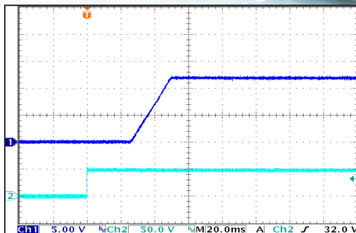
Figure 8: Turn-On Transient , at full resistive load and zero output capacitance initiated by Vin. Ch 1: Vout (5 V/div); Ch 2: Vin (50 V/div). Timescale: 20.0ms/div.
